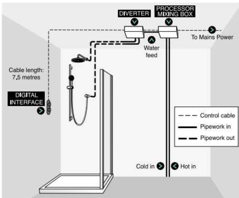
System Connection Diagram
