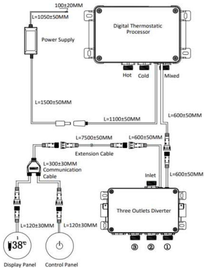
System Connection Diagram
