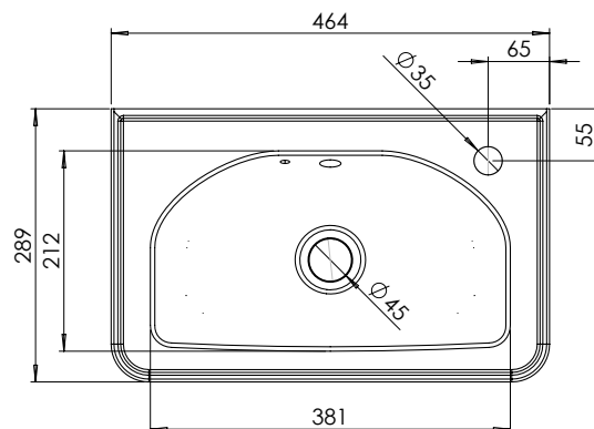
MS450CS (1 Tap Hole)
