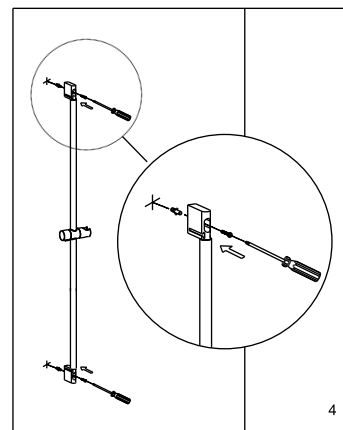
4. Fix the bar to the wall with anchors and screws.
