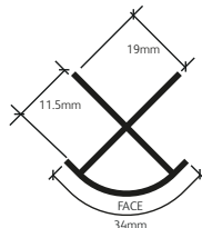
External Corner
