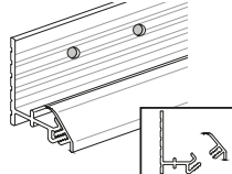
Sureseal Strip
