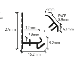
Sureseal Strip
