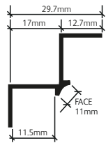
Internal Corner
