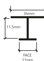
Joining Trim
