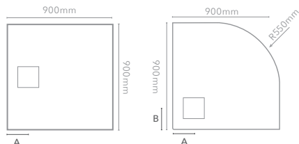
Square Tray
