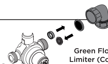
Yellow Flow Limiter (Hot)
