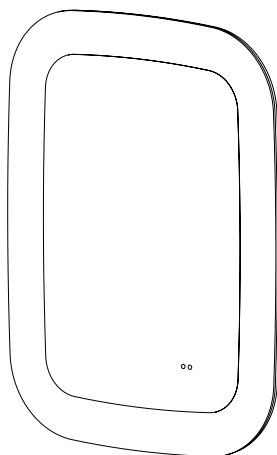
Cassini Curve
