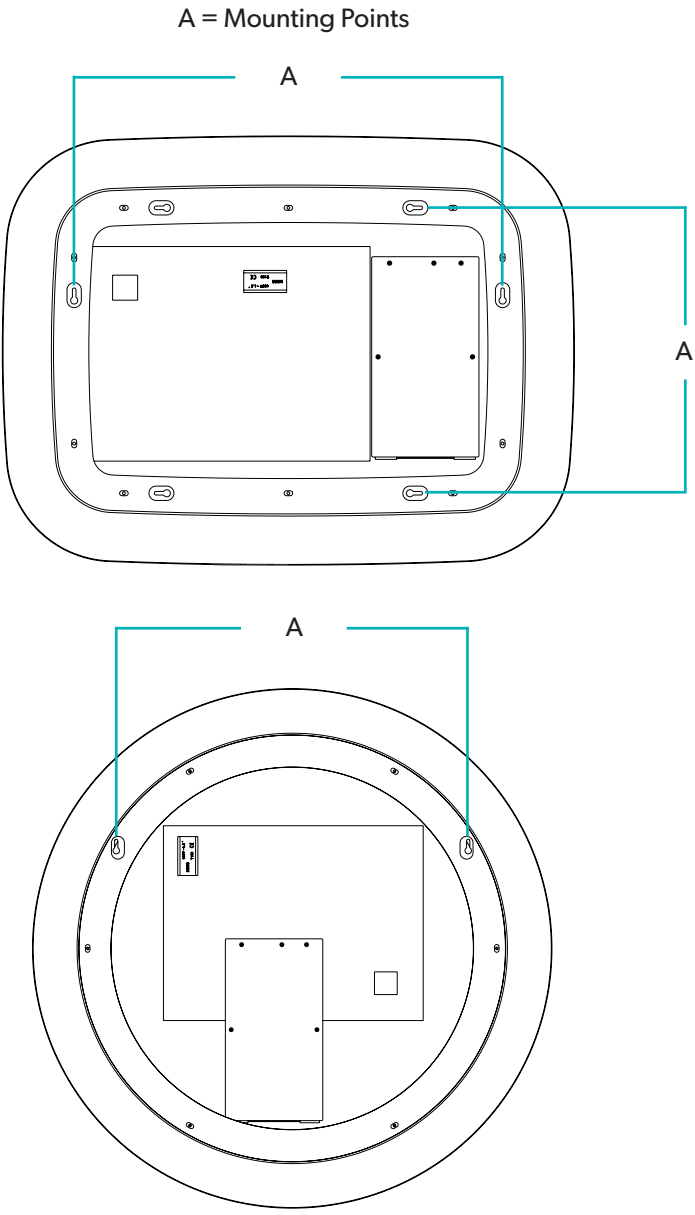
Fig 2. - Mounting points
