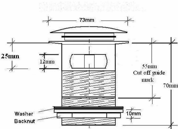
Marked as guide at 55mm in case the body needs length reduced
