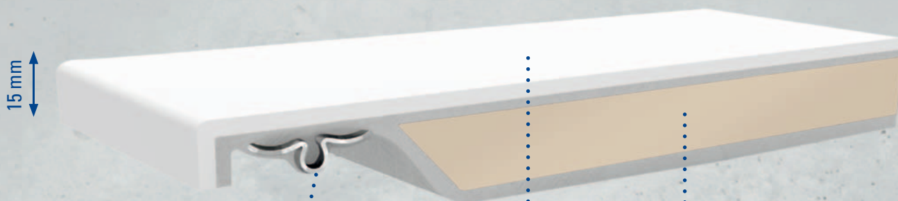
CROSS SECTION OF SHOWER TRAY, RIM HEIGHT 15 MM
