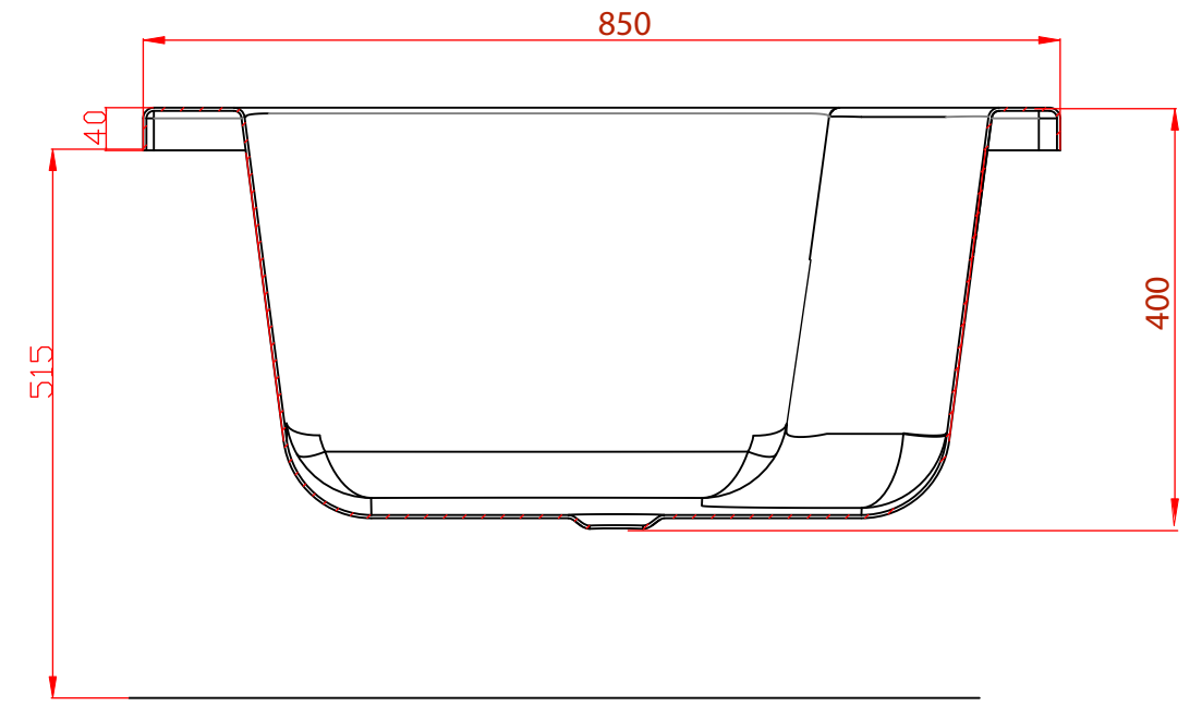
SECTION K-K SCALE 1 : 4
