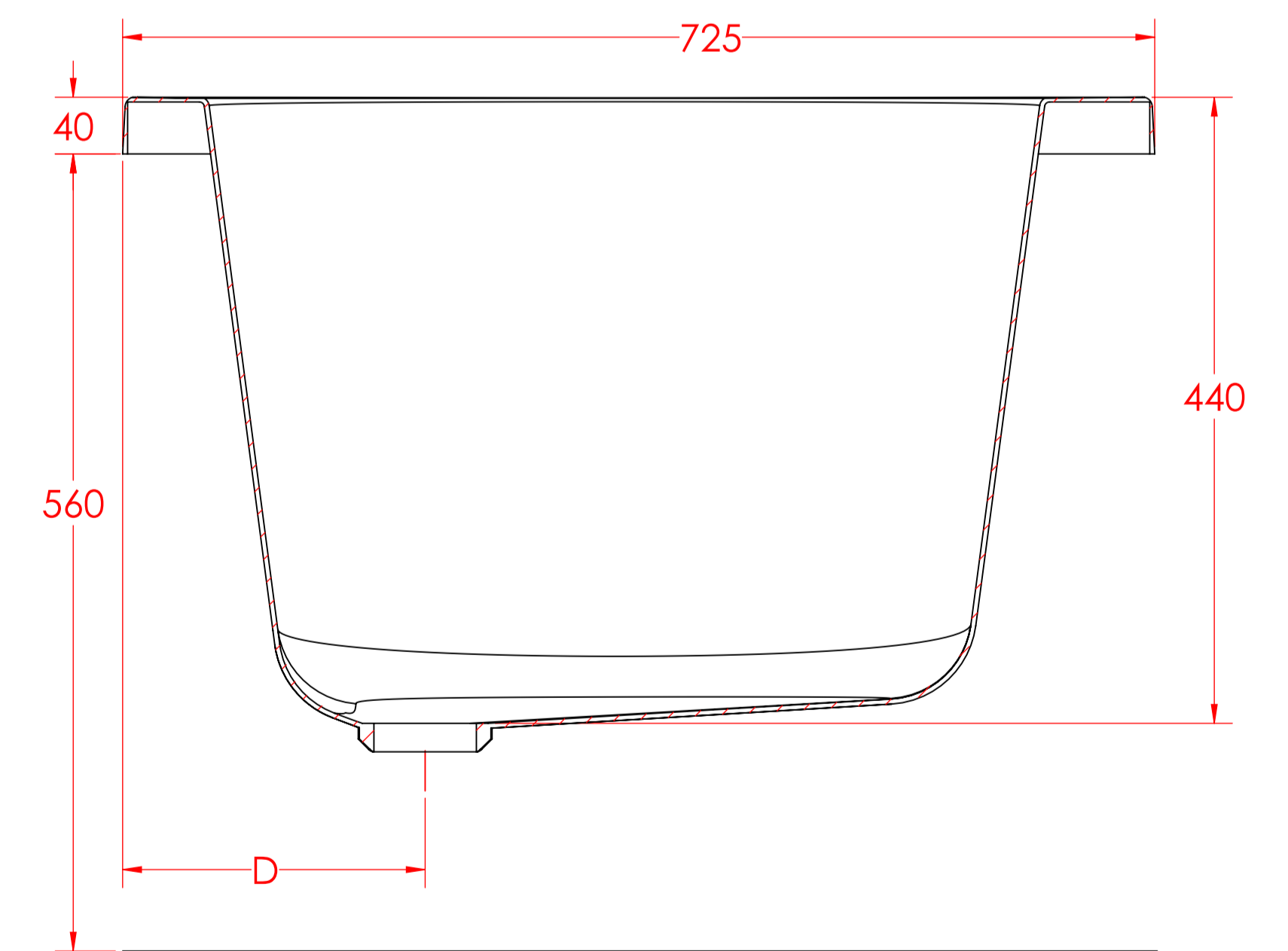
SECTION E-E SCALE 1 : 4
