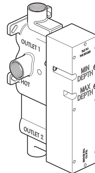
Valve with mortar guard
