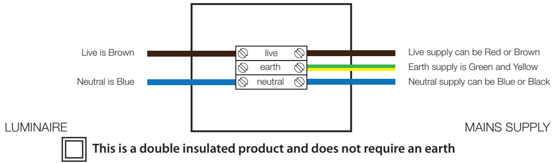
Wiring Diagram (Fig. B)
