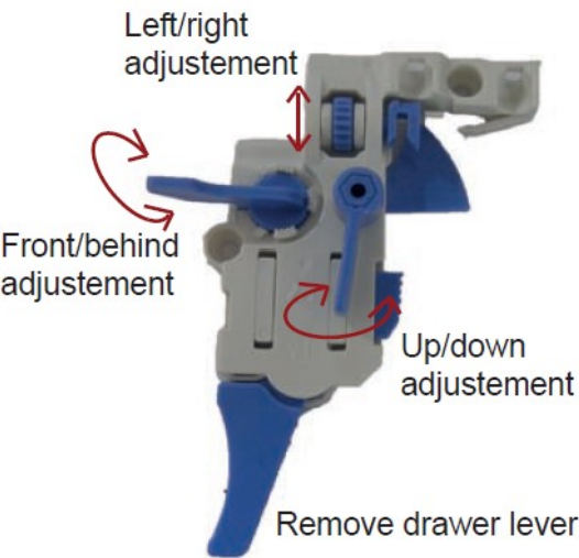
Drawer adjustment
