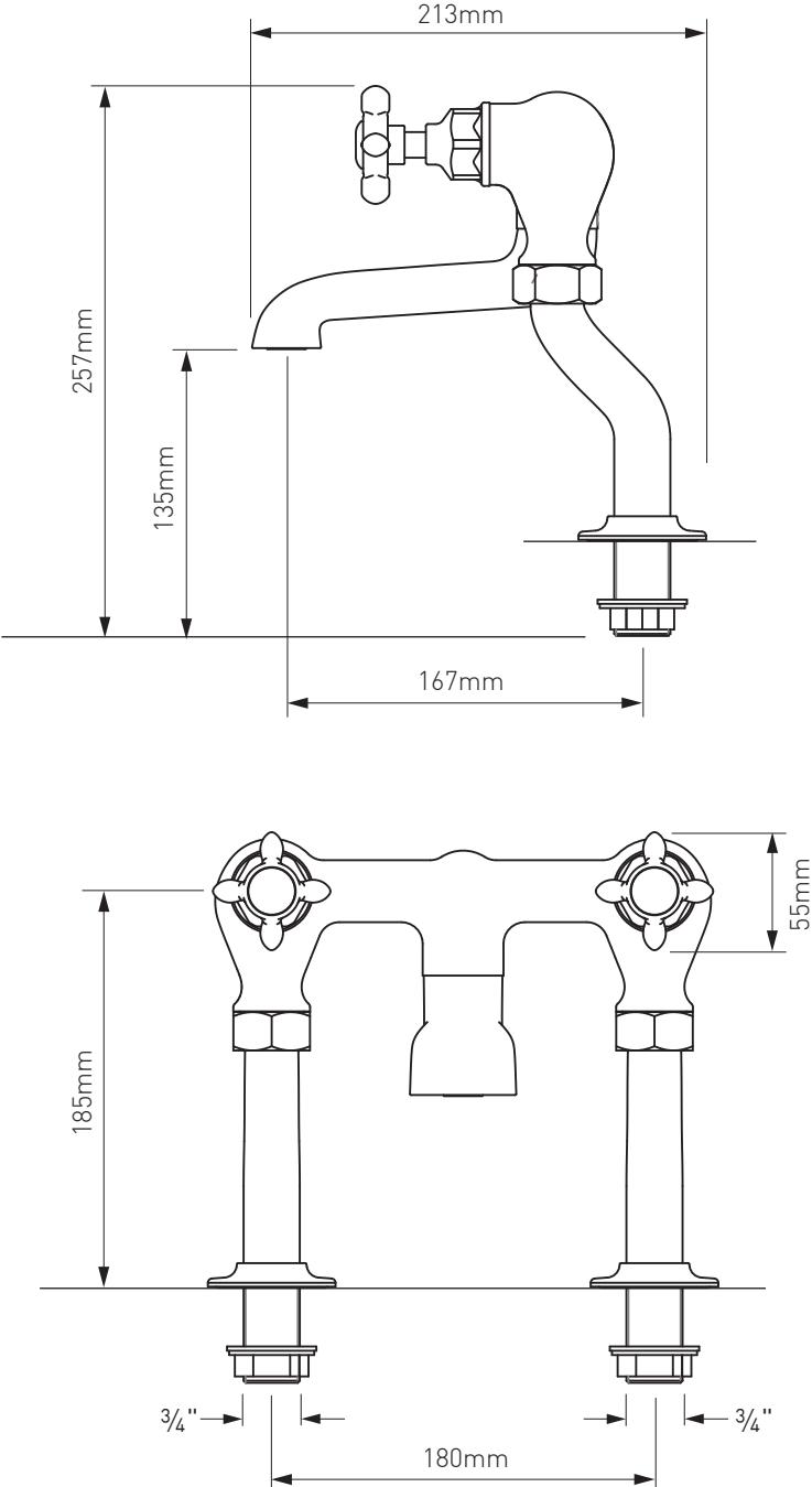
Dimensions - traditional handles
