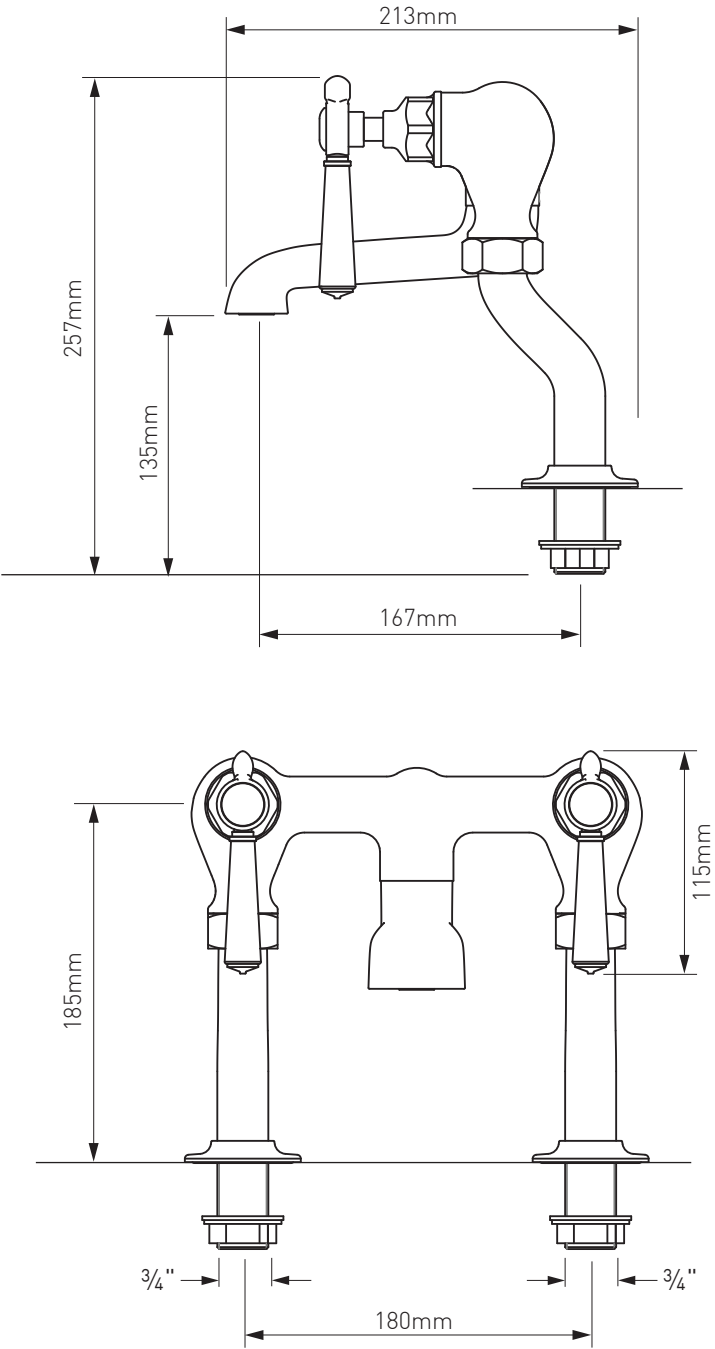
Dimensions - lever handles
