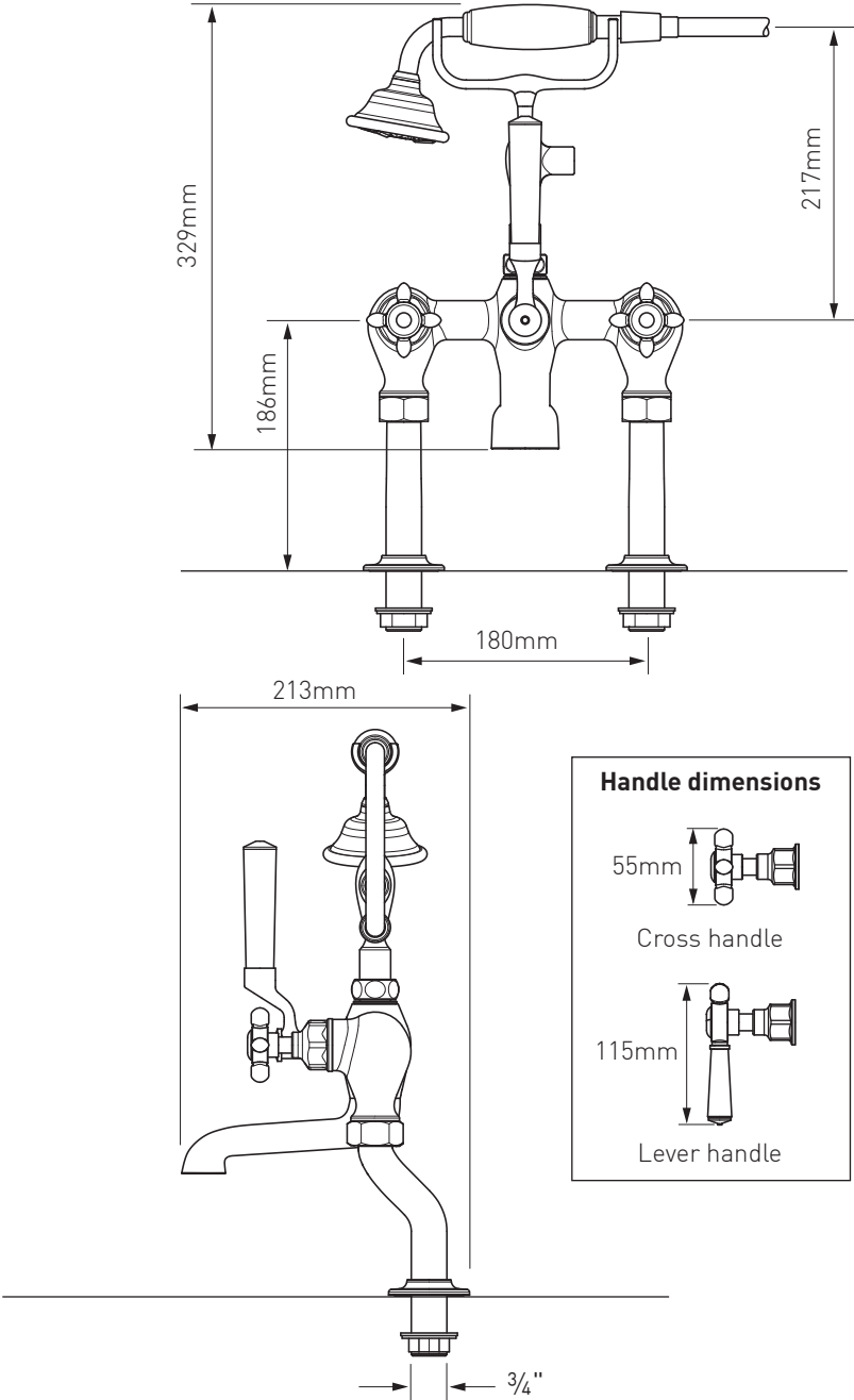
Cross handle shown
