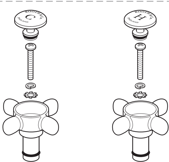
Cross handle option OR Lever handle option
