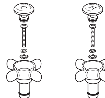
Cross handles with spring washer, lock washer, screw and screw cover
