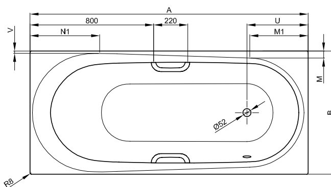
N° 1: foot end right, overflow front
