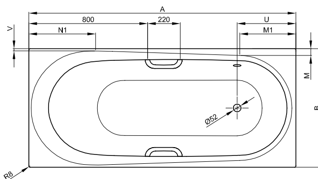
N° 2: foot end right, overflow rear
