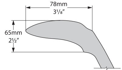
Rim Detail
